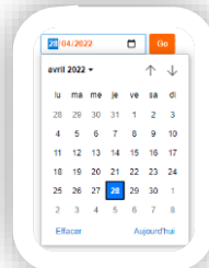
Calendar picker
