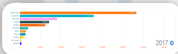
Bars race
